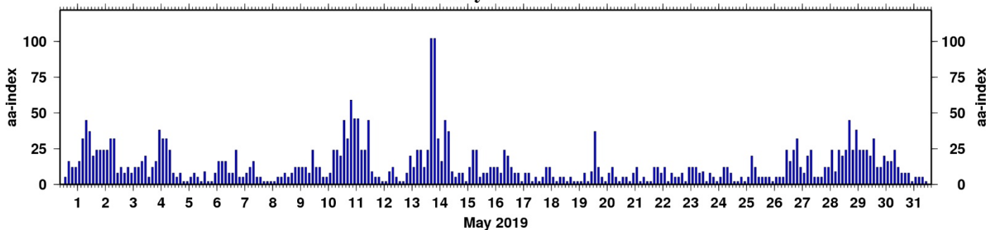
3-hourly aa -indices
