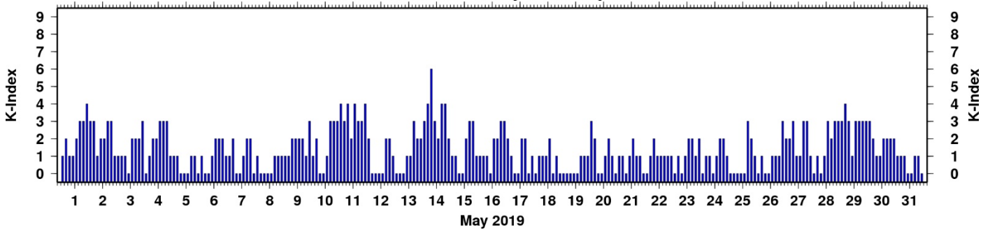
Eskdalemuir Observatory 3-hourly K-Indices
