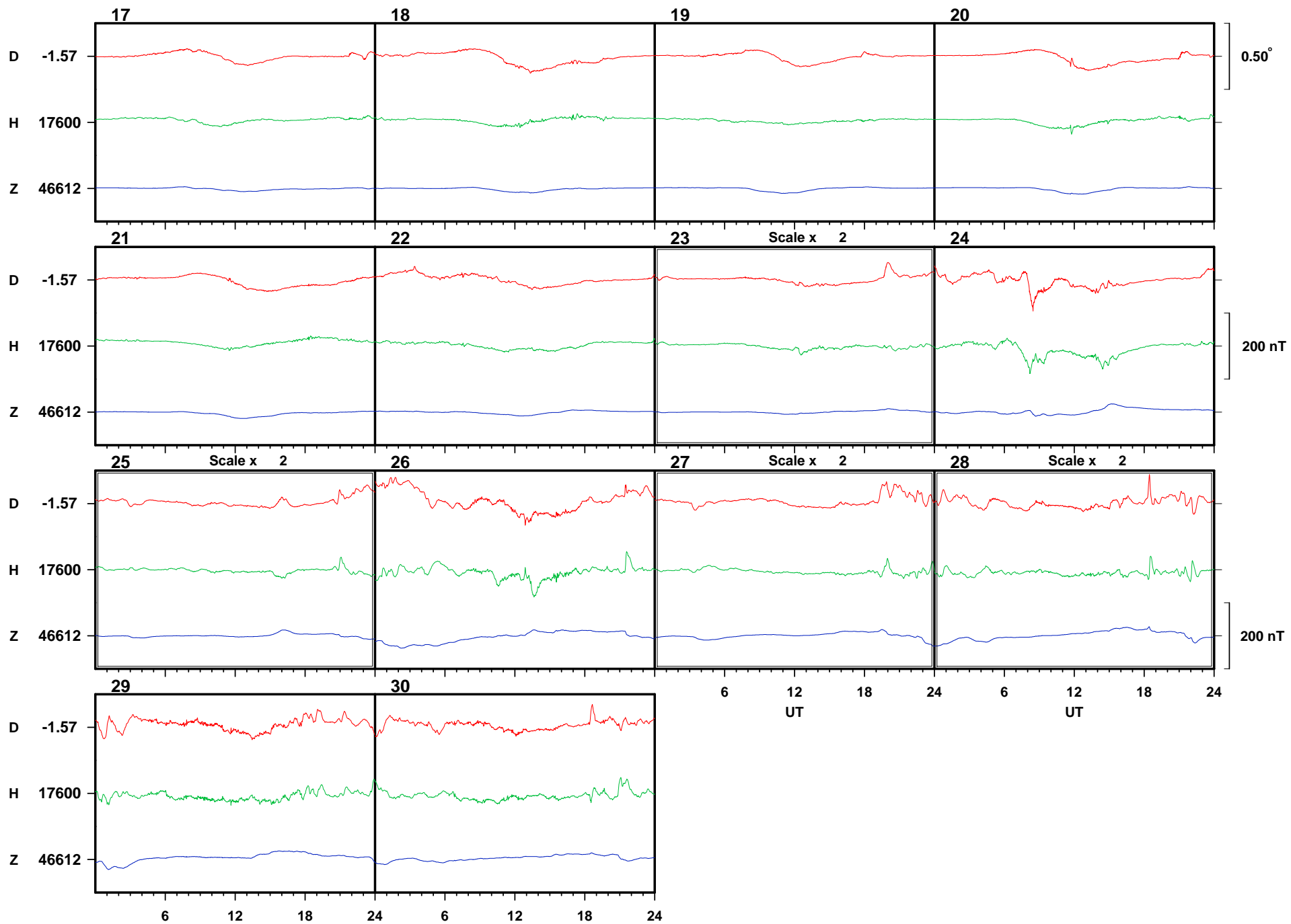
Eskdalemuir September 2020
